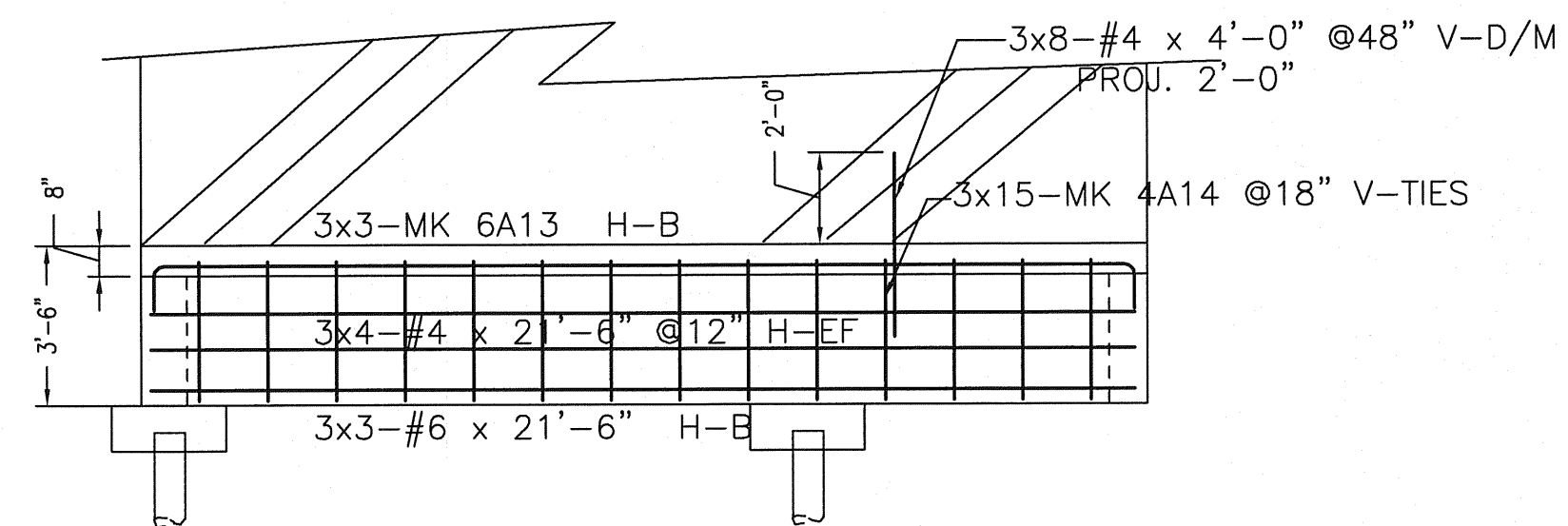
GB4 GRADE BEAM ELEVATION (3 LOCATIONS)
