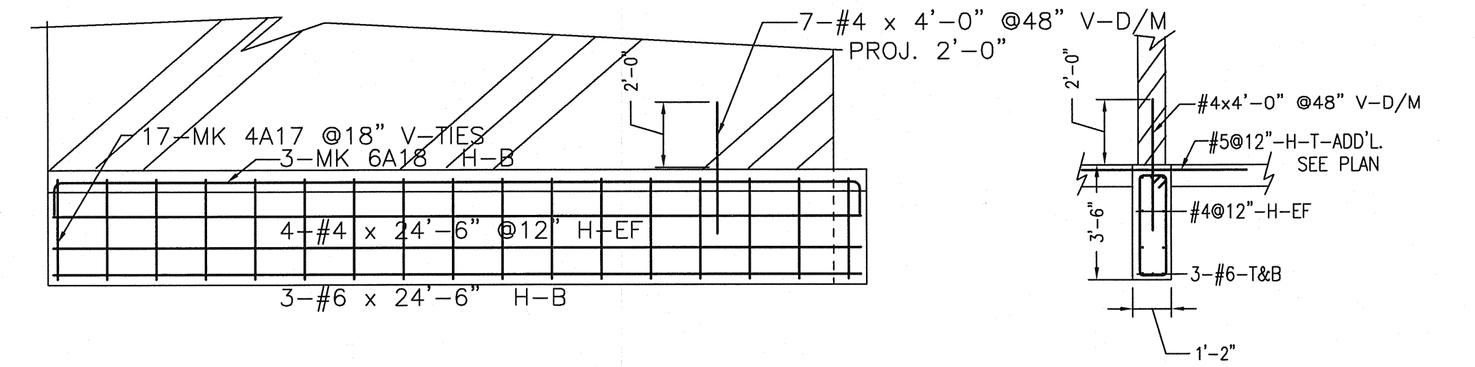
GB5 GRADE BEAM ELEVATION
