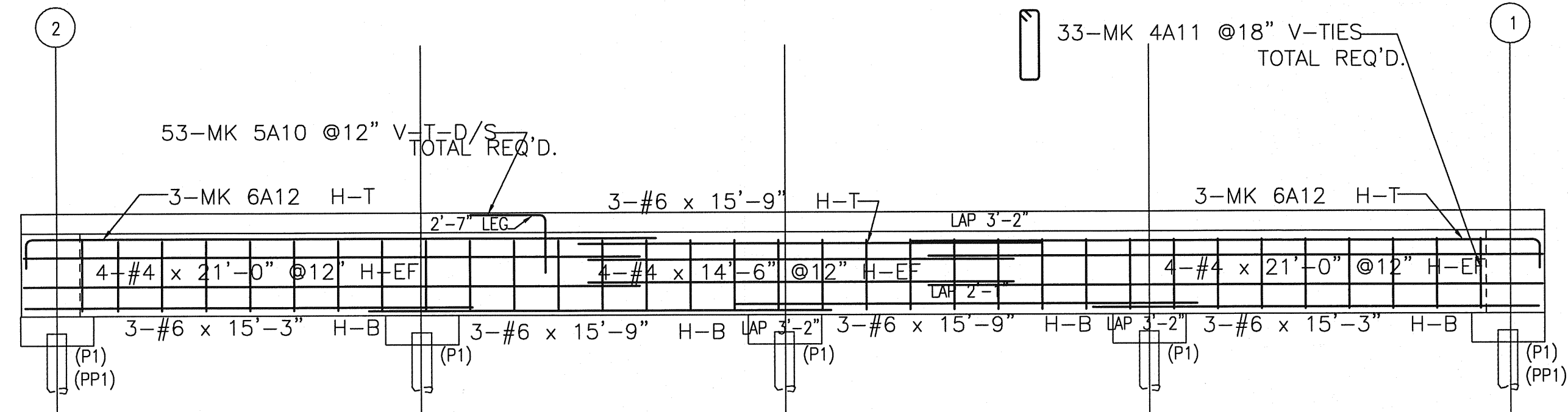
GB2A GRADE BEAM ELEVATION
