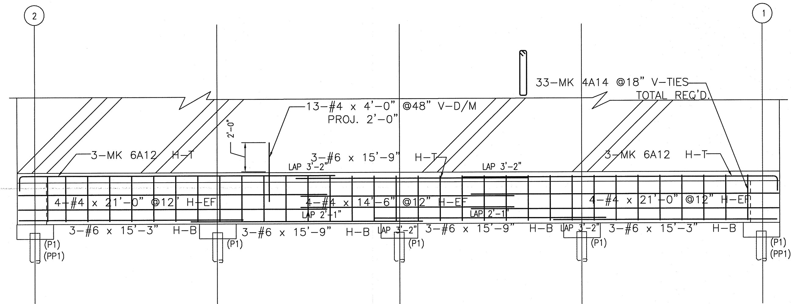
GB3 GRADE BEAM ELEVATION
