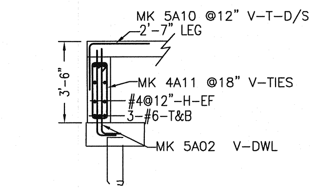
GB2 & GB2A GRADE BEAM SECTION
