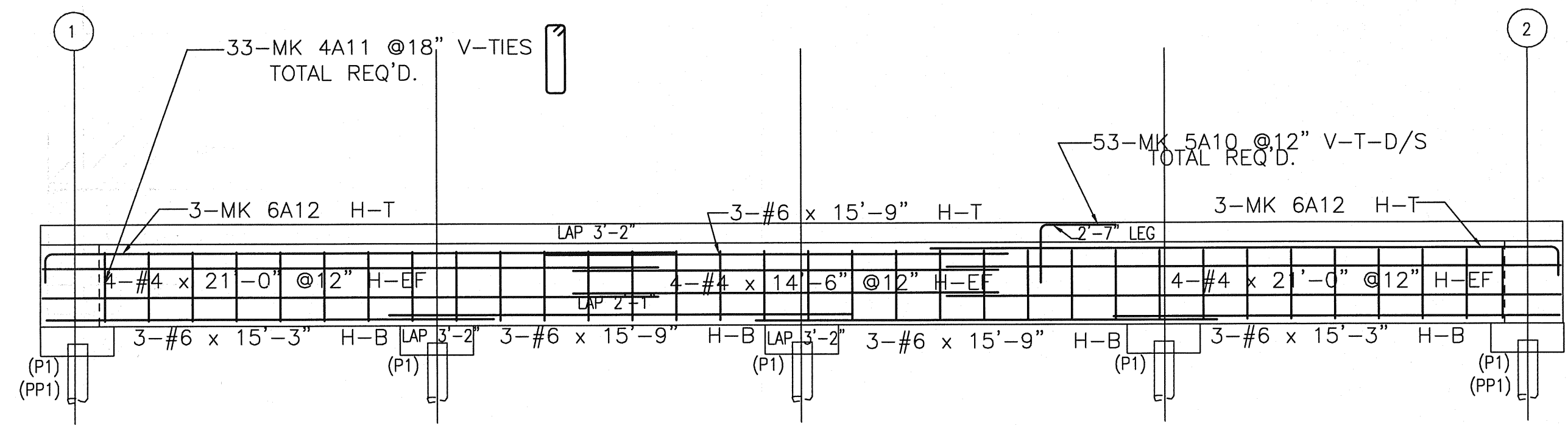
GB2 GRADE BEAM ELEVATION
